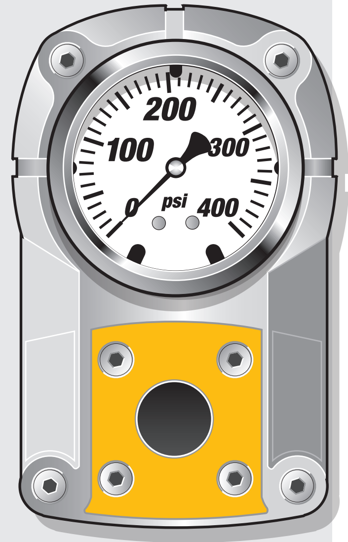
Integrated IC Swoop SMVC and Gauge Bezel Assembly
